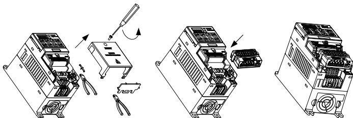
Figure 2-2 PDO-IO installation diagram
